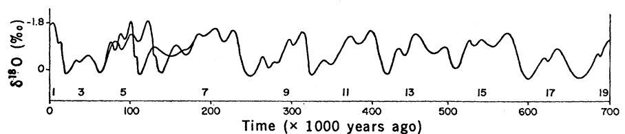
Fig. 4. Revised generalized paleotemperature curve and time scales D and E. The numbers above the abscissa identify deep-sea core stages.
