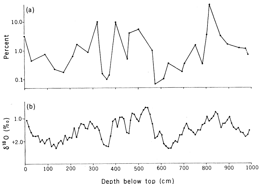
Fig. 2. Core 280 (North Atlantic, 34°57'N, 44°16'W). (a) Ratio of Epistominella umbonifera to E. exigua ; (b) oxygen isotopic record of Globorotalia inflata ; the data are from (30) and (15).
