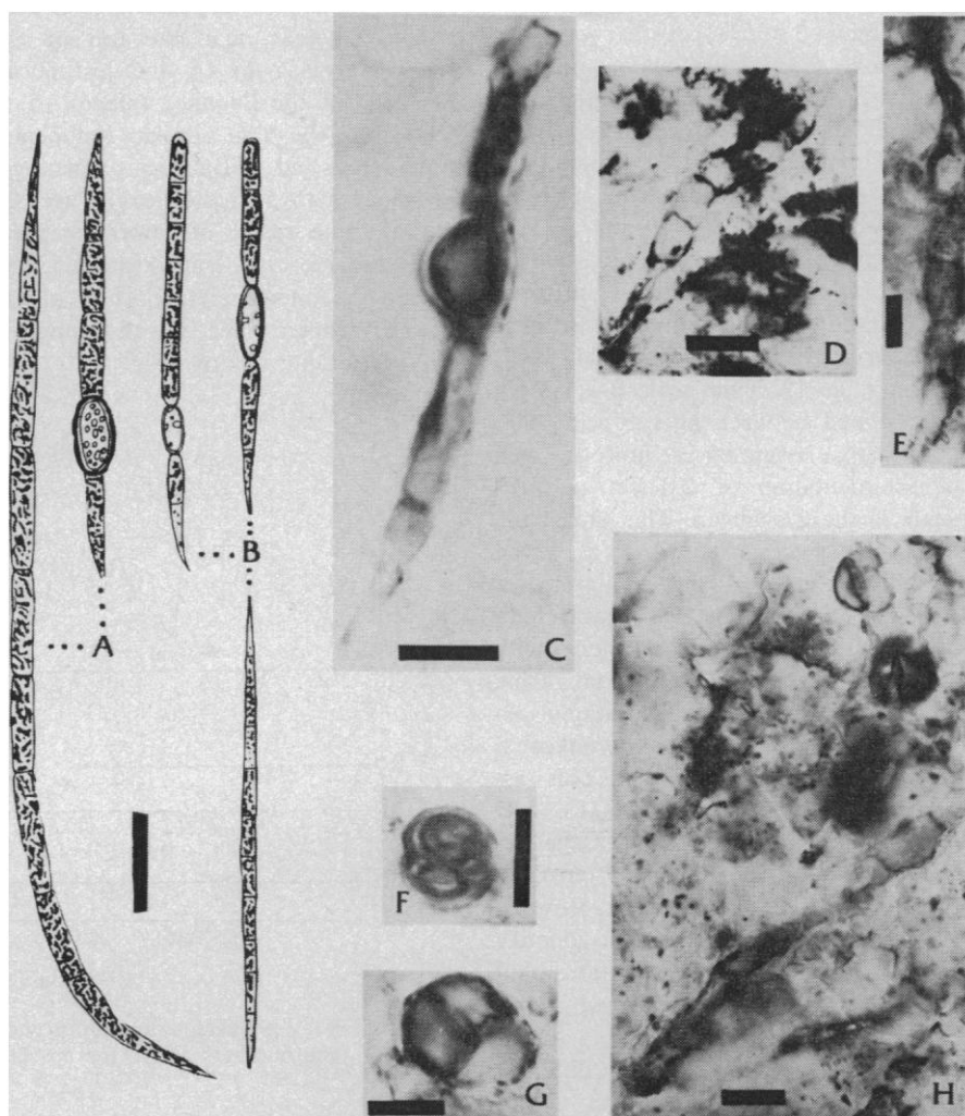
Fig. 1. (A and B) Comparison drawings modified from Desikachary (17) of the recent blue-green algae Raphidiopsis mediterranea and Raphidiopsis indica , respectively; scale bar, 10 \mu\text{m} . (C) New microfossil, Petraperha vivescenticula , showing enlarged akinete-like structure; scale bar, 10 \mu\text{m} . At the completion of this investigation the slide (No. TR1A) containing the type specimen will be deposited in the algal herbarium collection of the Academy of Natural Sciences of Philadelphia. (The specimen is marked with a diamond scribe.) (D and E) Broken filamentous forms; scale bar, 10 \mu\text{m} . (F and G) Simple round forms which could represent coccoid blue-green algae; scale bar, 5 \mu\text{m} . (H) Assemblage of a broken filament and round forms; scale bar, 10 \mu\text{m} . All the Transvaal photomicrographs are from petrographic thin sections.
