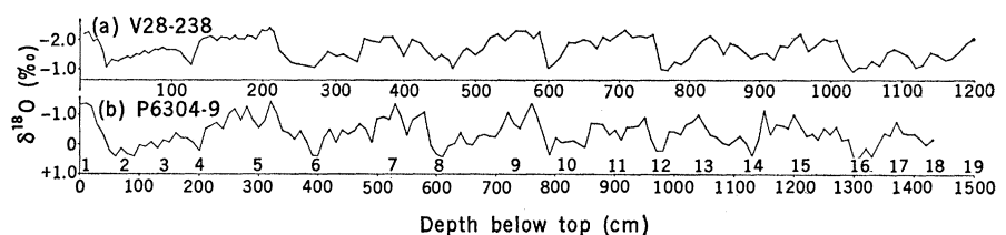
Fig. 1. Cores (a) V28-238 (western equatorial Pacific, 1°1'N, 160°29'E) and (b) P6304-9 (Caribbean sea, 14°57'N, 69°20'W); oxygen isotopic record of Globigerinoides sacculifera during Brunhes epoch [see (4) for pre-Brunhes record of core V28-238]. The horizontal scale of core V28-238 has been adjusted to make the peak of stage 5 coincide with that of core P6304-9. The numbers above the abscissa identify deep-sea core stages.
