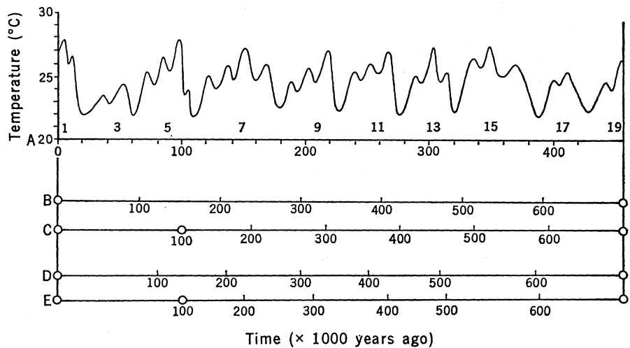
Fig. 3. Generalized paleotemperature curve of 1972 (2) with four possible time scales (B to E). The numbers above the abscissa for curve A identify deep-sea core stages.
